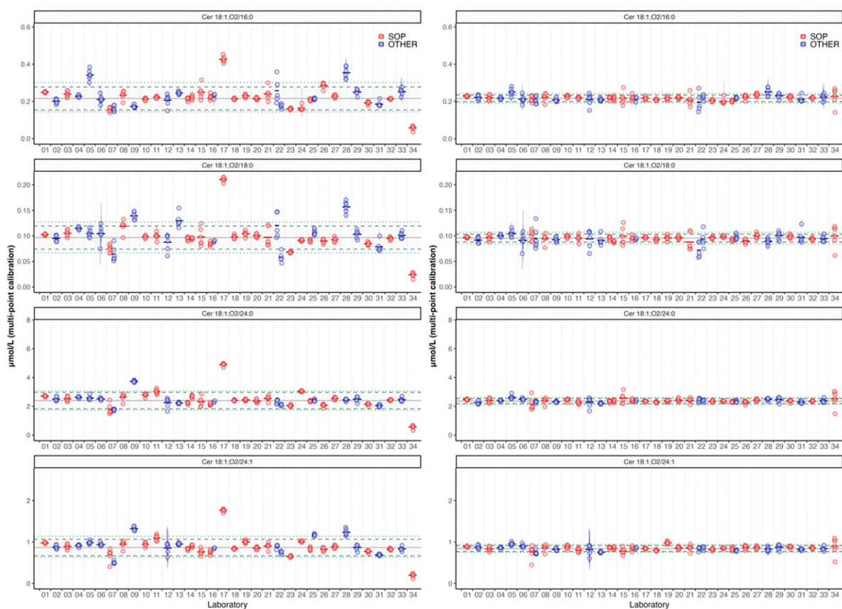
Supplementary Figure 9. Re-calibration of DB using SRM 1950 after multi-point calibration. All datasets are shown here, while the indicated %CVs were calculated after exclusion of outliers (see Fig. 1 and text). Source data are provided as Source Data file.
