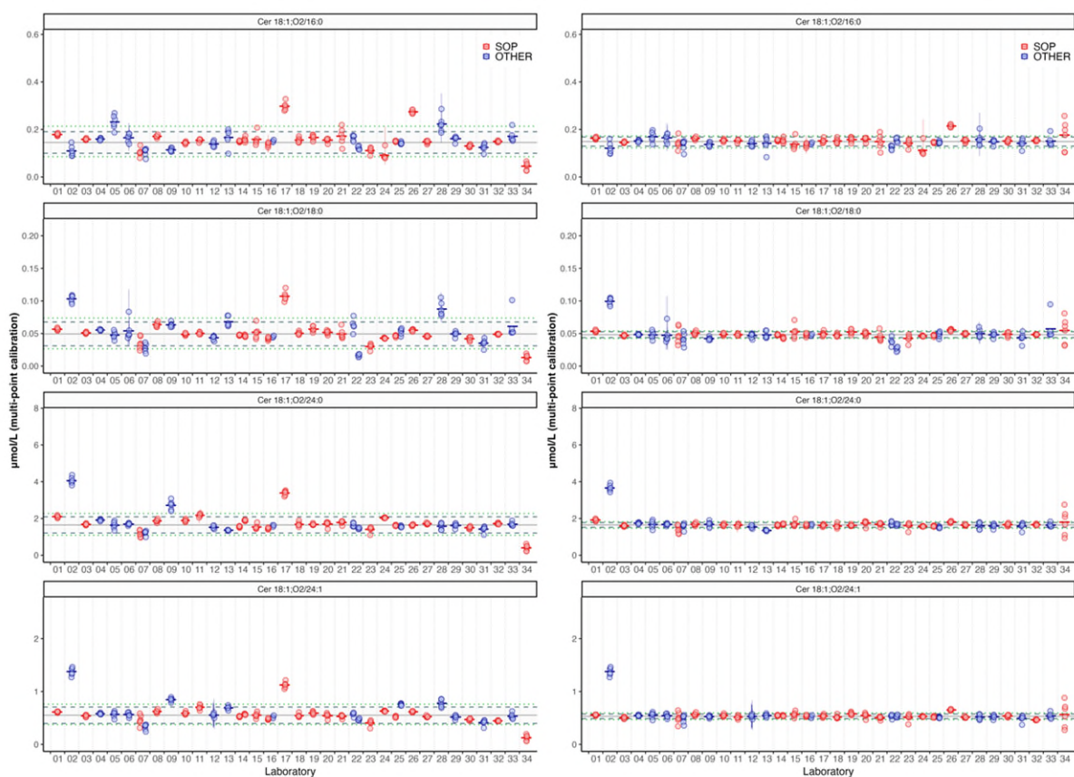
Supplementary Figure 10. Re-calibration of YAA using SRM 1950 after multi-point calibration. All datasets are shown here, while the indicated %CVs were calculated after exclusion of outliers (see Fig. 1 and text).
