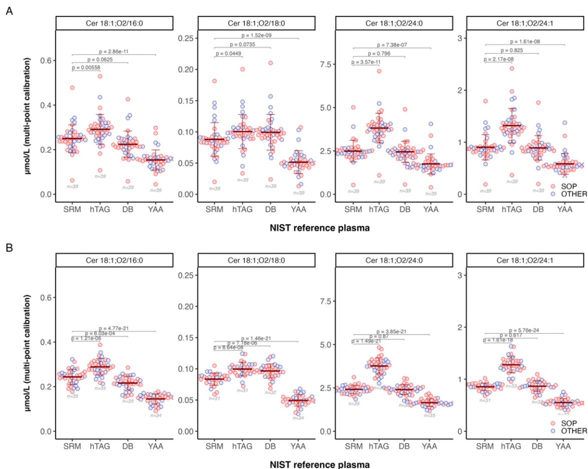
Supplementary Figure 4 – Concentration values of ceramides in NIST SRM 1950 and the suite of human plasma RM contained in RM 8231 of the full (A) and outlier-filtered (B) dataset.
