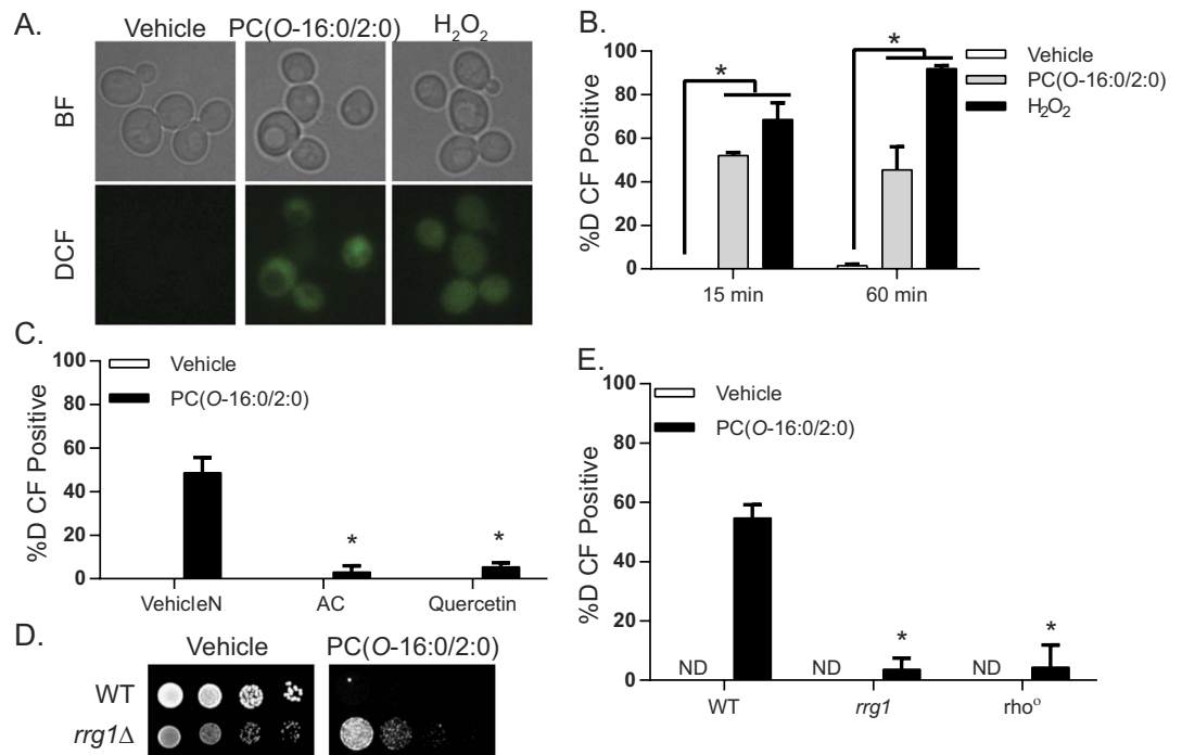
Figure 2. Mitochondria are the major source of ROS production in PC(O-16:0/2:0) treated cells. (A) H 2 -DCFDA fluorescence is increased in PC(O-16:0/2:0) treated cells. Wild type (BY4741) cells were grown to mid log in YPD and subsequently treated with Vehicle (0.2% Ethanol), PC(O-16:0/2:0) (20 μM) or H 2 O 2 (0.8 mM) for t = 15 or 60 min prior to labelling with H 2 -DCFDA (10 μM). Representative brightfield (BF) and H 2 -DCFDA (DCF) images from t = 15 min are shown. (B) Quantifications of H 2 -DCFDA positive cells at the indicated time points from at least three independent experiments where a minimum of 150 cells were counted. Error bars = SD, (*p < 0.01, Kruskal-Wallis test). (C) Antioxidants reduce H 2 -DCFDA fluorescence. Wild type (BY4741) cells were grown to mid log in YPD with or without n-acetyl cysteine (NAC 20 mM, pH 7.5) or quercetin (300 μM) and subsequently treated with PC(O-16:0/2:0) (20 μM, 15 min) and labeled with H 2 -DCFDA (10 μM) and positive cells were quantified. A minimum of 150 cells from three independent experiments were counted. Error bars = SEM, (*p < 0.01, Kruskal-Wallis test). (D) Inhibition of ROS production reduces PC(O-16:0/2:0) toxicity. Sensitivity of wild type (WT, BY4741) and rrg1 Δ (YKB3911) strains were assessed by examining growth on plates containing vehicle (Ethanol, EtOH) or PC(O-16:0/2:0) (7 μg/mL or 13.4 μM) at 30 °C for 2 days. Representative image from 3 experiments is shown. (E) Mitochondrial respiration is required for ROS production in PC(O-16:0/2:0) treated cells. Wild type (BY4741), rrg1 Δ (YKB3911), rho o (YKB3925) cells were grown to mid log, treated with PC(O-16:0/2:0) (20 μM, 15 min) and labeled with H 2 -DCFDA (10 μM). A minimum of 150 cells from three independent experiments were counted. Error bars = SEM, (*p < 0.05, Kruskal-Wallis test). ND – not detected.
